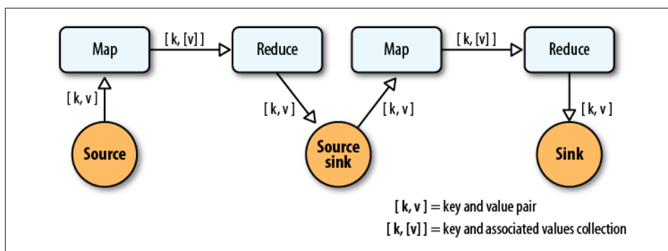
Figure 16-11. Counting and sorting in MapReduce
