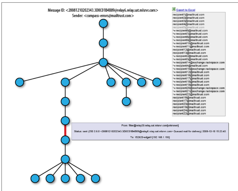
Figure 16-10. Data tree
